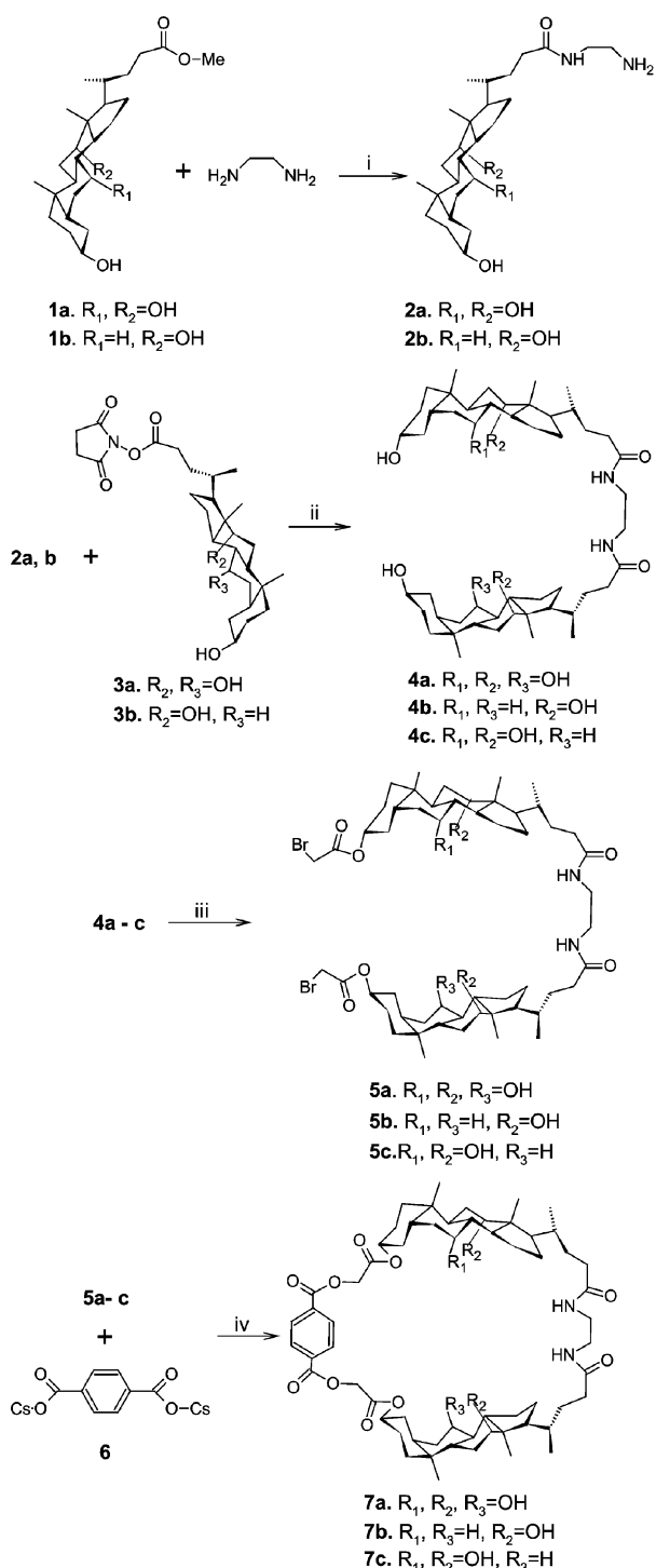
Scheme 1 Reagents and conditions (and yields): i, CH 3 OH, rt, 48 h, (98%); ii, DMF, rt, 24 h, 4a (96%), 4b (95%), 4c (96%); iii, BrCH 2 COBr, anhydrous K 2 CO 3 , CHCl 3 , 55–60 °C, 10 min, 5a (70%), 5b (75%), 5c (73%); iv, DMF, 12 h, rt, 7a (95%), 7b (85%), 7c (87%).
